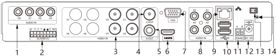
Figure 1-2 Real panel
